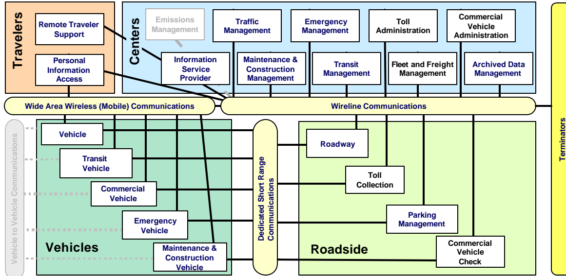
Youngstown-Warren Regional ITS Architecture "Sausage Diagram"
